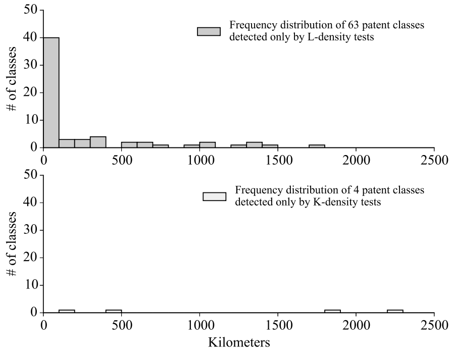
Figure D2: Frequency distributions of patent classes for the distances at which the members in \mathcal{A}_{\text{KD}\setminus\text{LD}} and \mathcal{A}_{\text{LD}\setminus\text{KD}} initially display localization (median citation distance). The bars in dark grey (resp., light grey) are the frequencies of localized patent classes detected only by the L -density (resp., K -density) tests.
